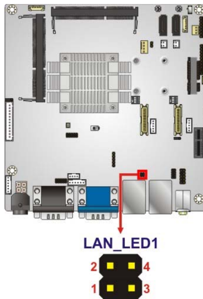
Figure 3-16: LAN Active LED Connector Location
