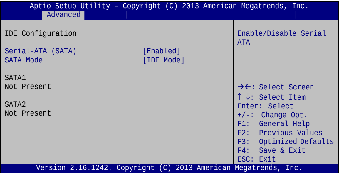
BIOS Menu 12: IDE Configuration
