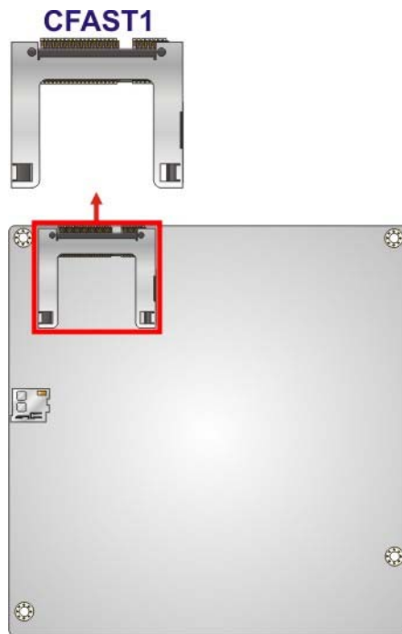
Figure 3-9: CFast Card Slot Location
