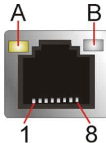
Figure 3-36: Ethernet Connector
