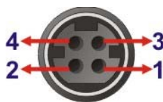
Figure 3-34: 9 V ~ 26 V DC In Connector
