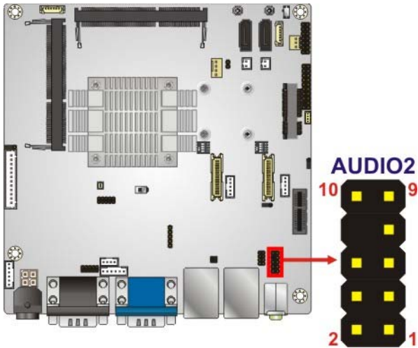
Figure 3-5: Audio Connector Location
