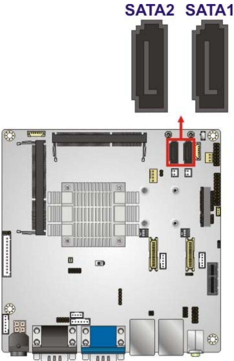
Figure 3-23: SATA 3Gb/s Drive Connector Locations
