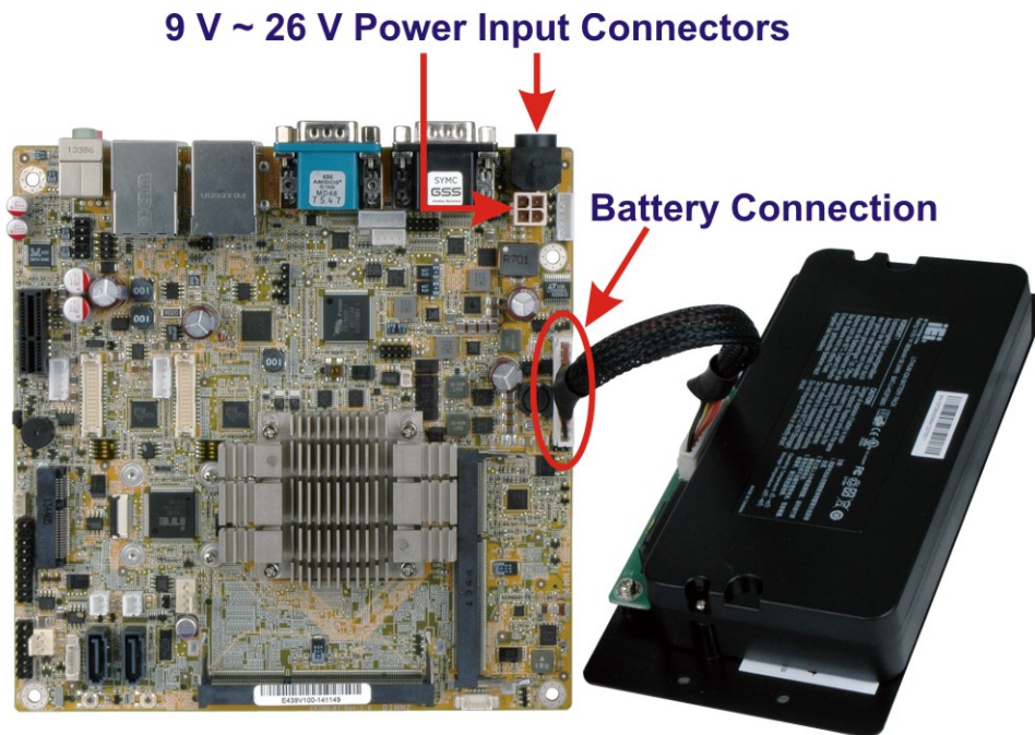
Figure 4-10: UPS Installation
