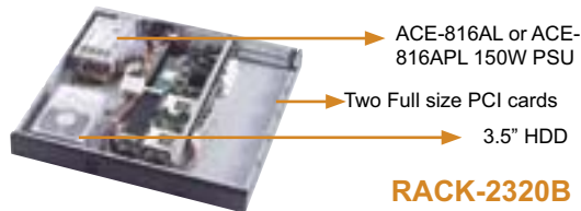
RACK-2320B
